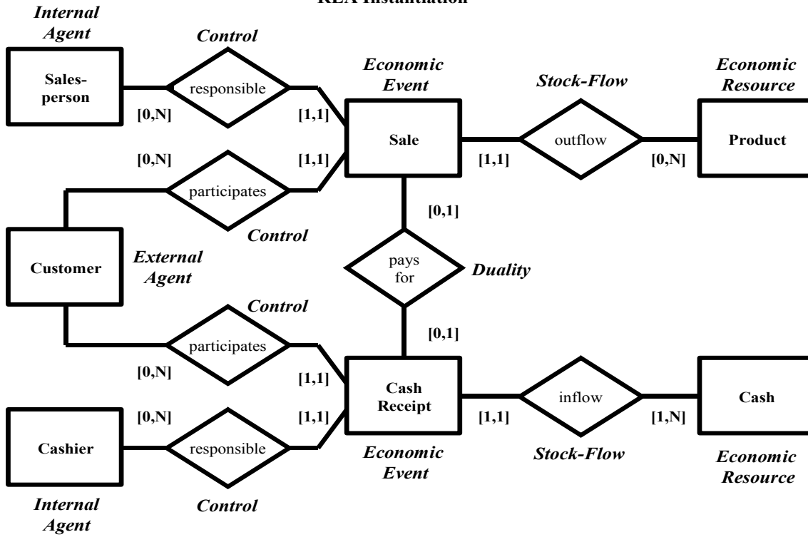
FIGURE 4 REA Instantiation
