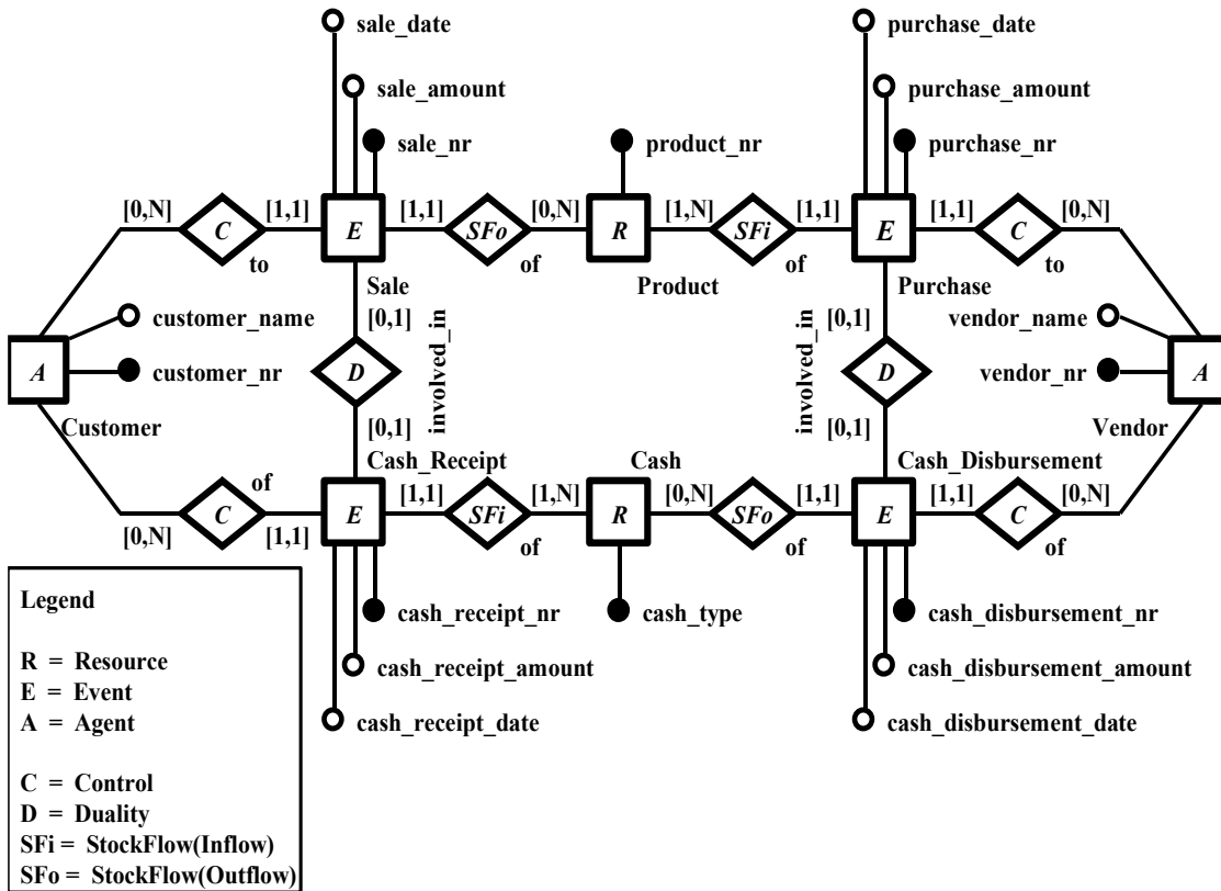
FIGURE 7 REA Example
